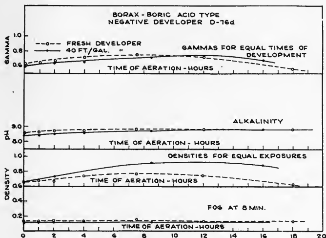
FIG. 3. Effect of aeration of a borax-boric acid negative developer (Formula D-76d).
